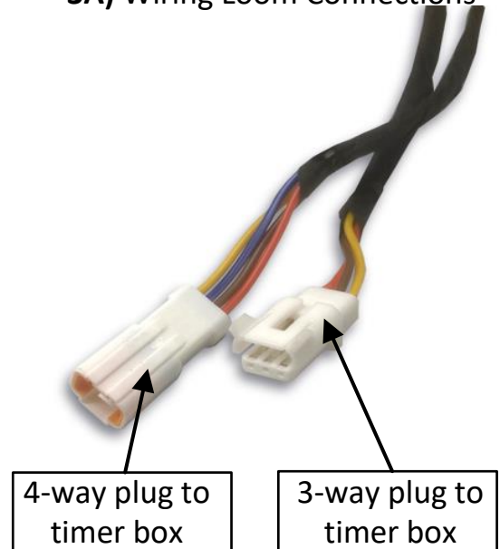
3A) Wiring Loom Connections
